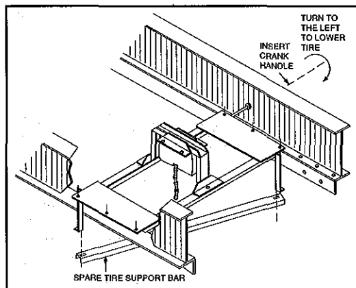
Spare Tire Center
